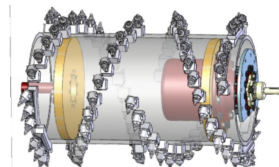
Keystone's Complete Cutter Drive Conversion with Replacement Drum
