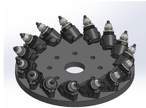
Rotary Plate with Standard Carbide Tools
