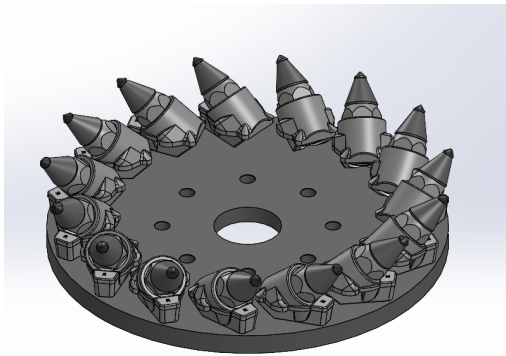
Rotary Plate with PCD Diamond Tools
