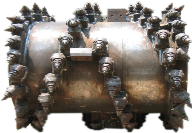
Easy Screw Quick-Change System for Skid Steer Milling Attachments
