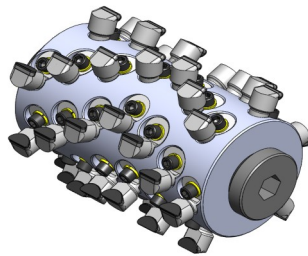
7"+ Diameter drum system for walk behind grooving and grinding machines
