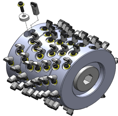
10"+ Diameter drum system for truck mounted grooving and grinding machines
