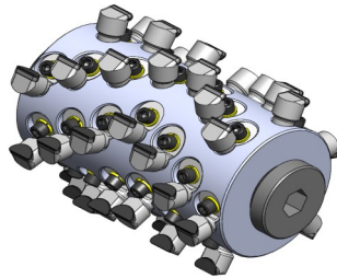
7"+ diameter drum for walk behind grinding machines
