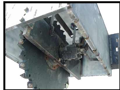
Sawing Head- Cuts 12" deep at 1.5" wide
