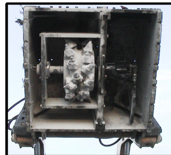
Longitudinal Joint Repair- V-Head Drum
