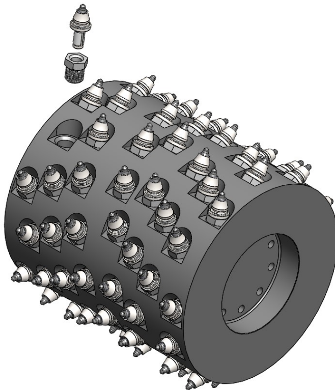
Standard Carbide Tool and Insert
